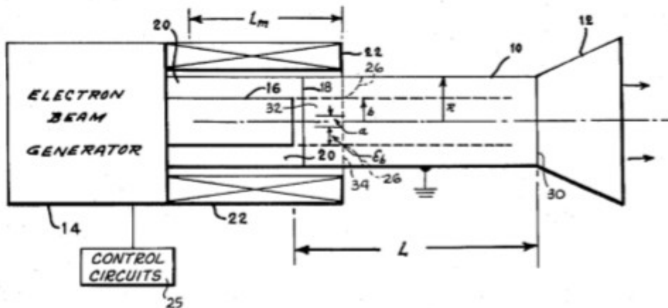
Figure 6. Patent 4345220. Vircator.
