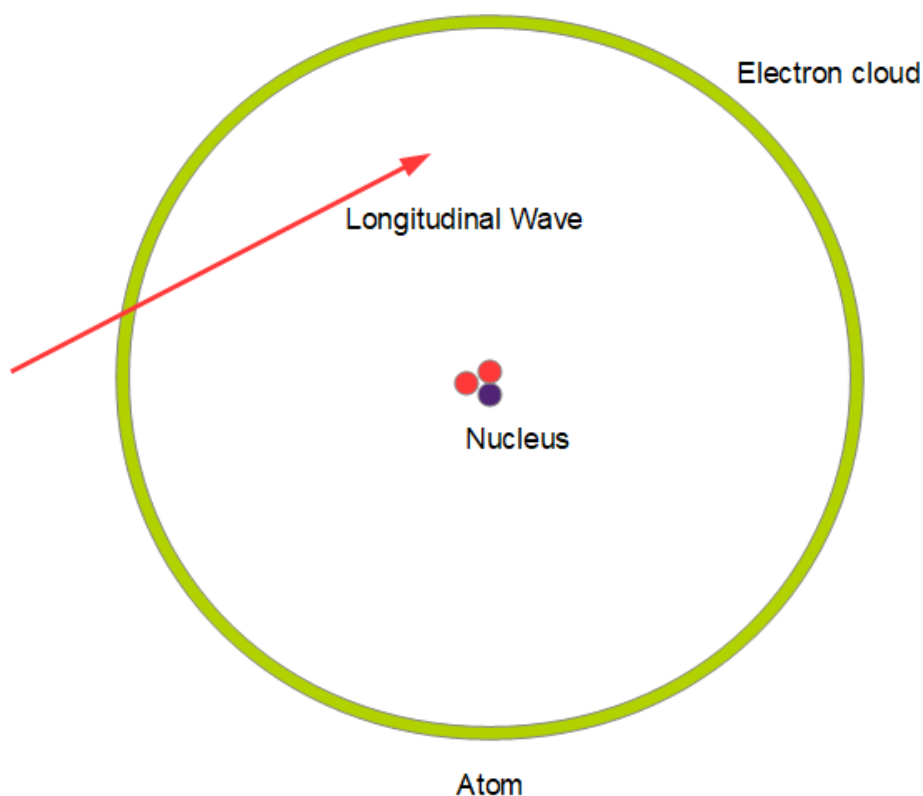
Figure 3. How does a scalar wave penetrate through buildings and houses? A scalar wave is incredibly small in its cross-section. Theoretically, it is a one-dimensional line, and the line has no measurable thickness. This means it can travel through many atoms and never hit anything.
