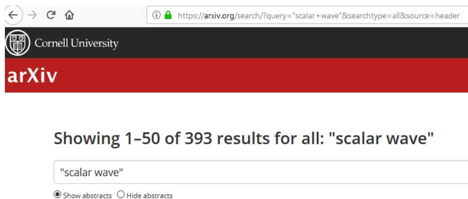
Figure 5. Arxiv.org – search for “scalar waves”
