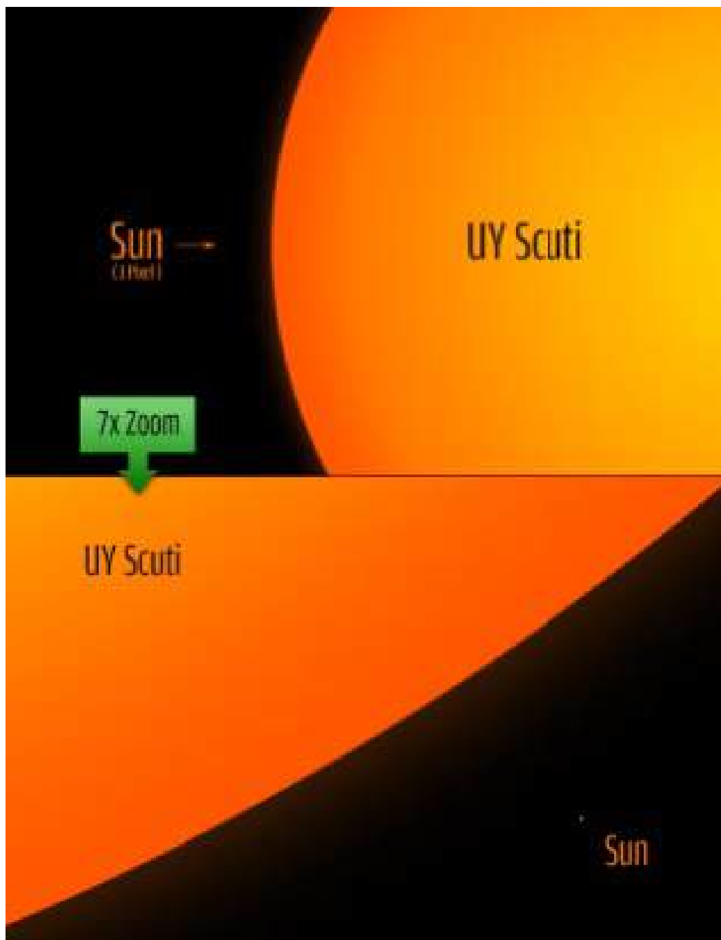
The sun compared to UY Scuti
