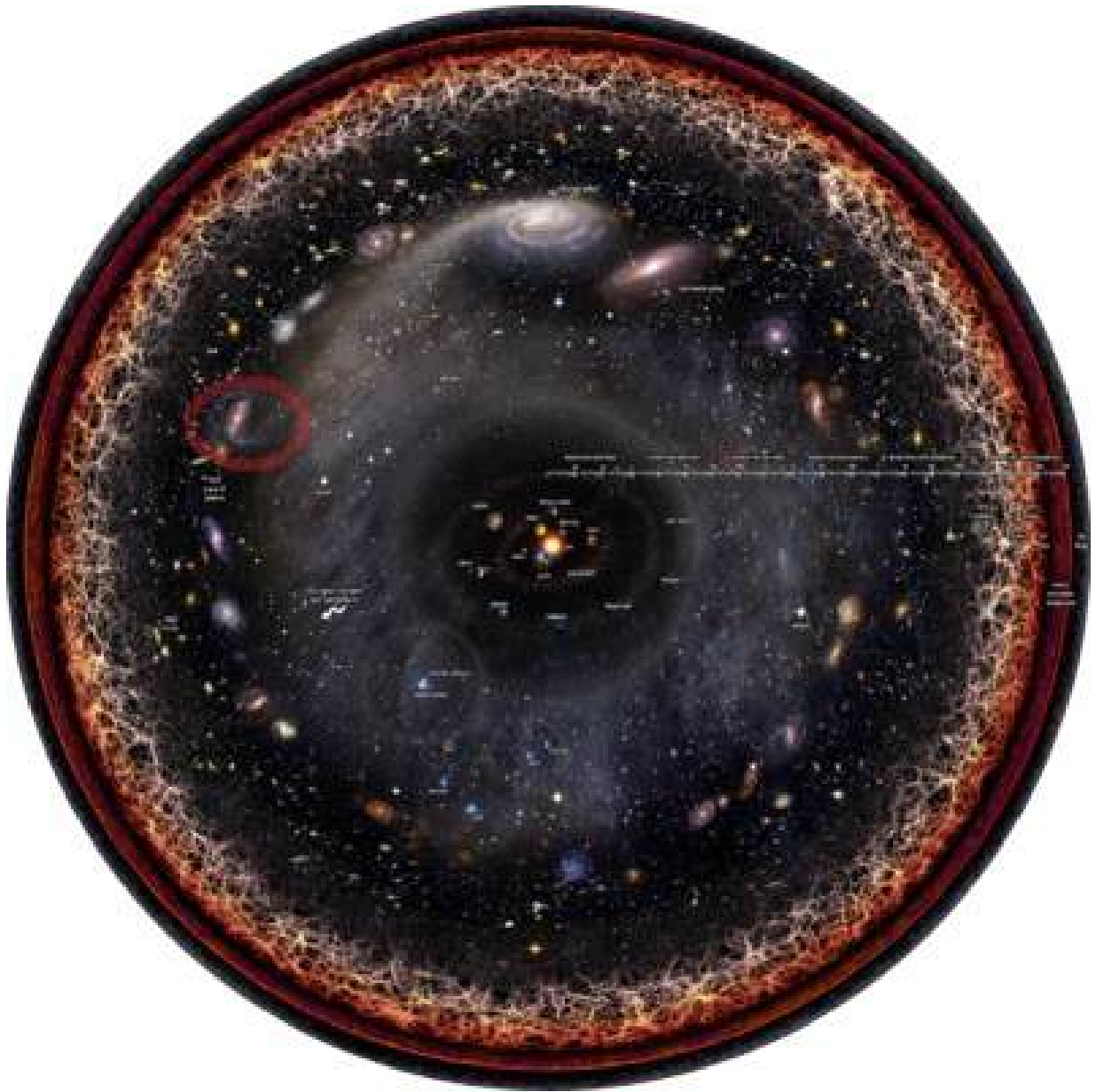
This is the observable universe so far and the red circle is the cluster of galaxies called "Laniakea".
